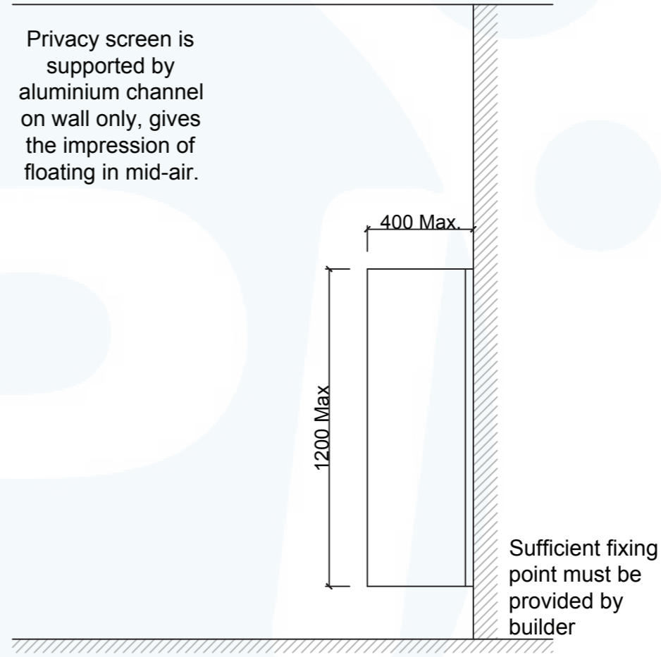
○ Wall Mounted Detail for Acrylic sheet option only
